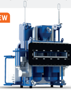
ELECTRIC-POWERED HUSQVARNA BLASTRAC EBE 900VMB 2×22 kW, 400 V, 125 A, working speed 0.5–10 m/min, working width 890 mm, 880 kg.
