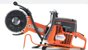
PETROL-POWERED HUSQVARNA K 760 CUT-N-BREAK 74 cc, 3.7 kW, 11.1 kg, blade size 230 mm, cutting depth 400 mm.
