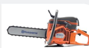
PETROL-POWERED HUSQVARNA K 970 CHAIN 94 cc, 4.8 kW, 9.7 kg, bar size 350 mm, cutting depth 400 mm.
